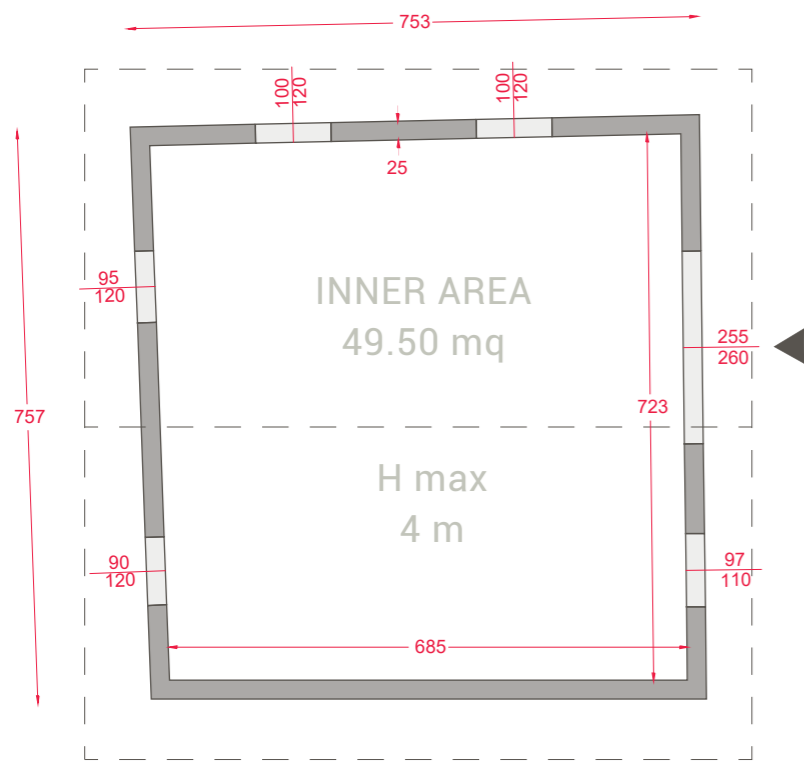
GROUND FLOOR - INITIAL STATUS
