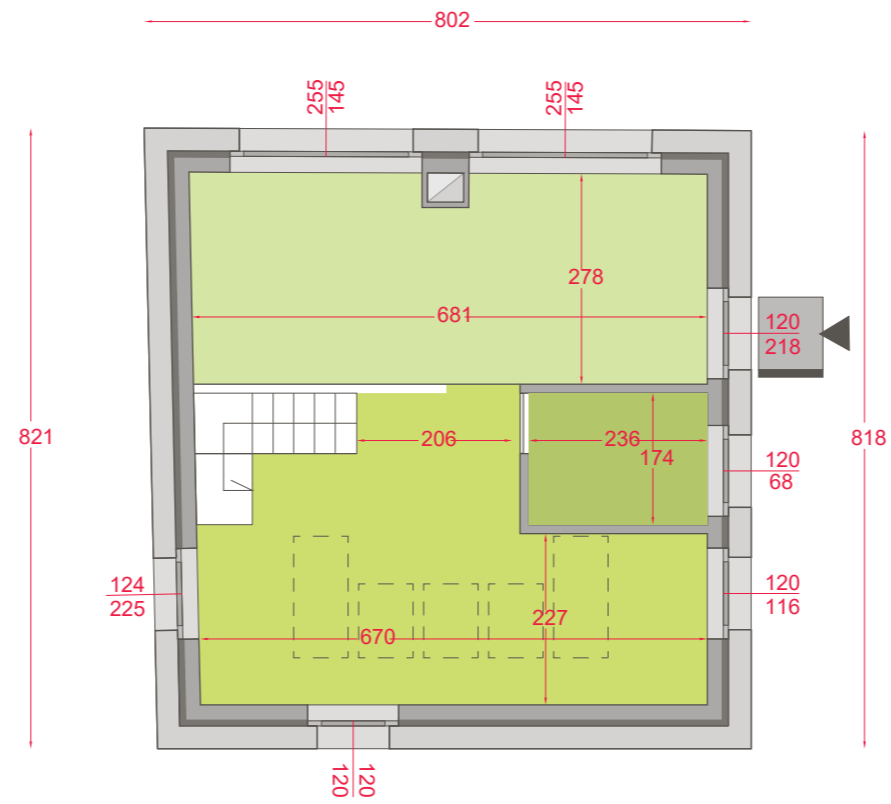
GROUND FLOOR - PROJECT STATUS
