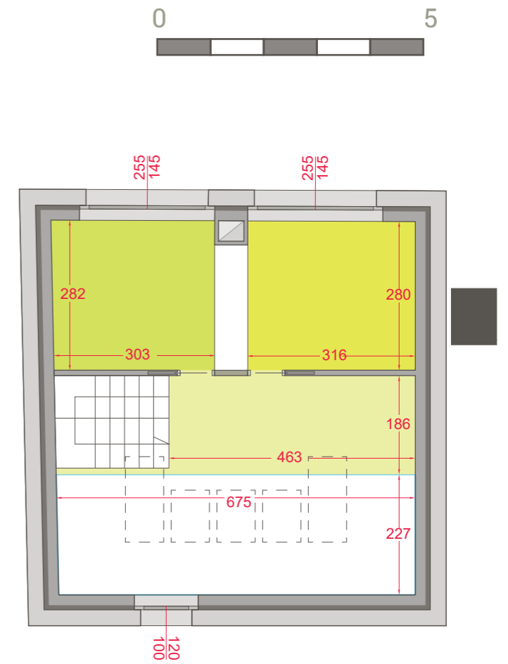
FIRST FLOOR - PROJECT STATUS
